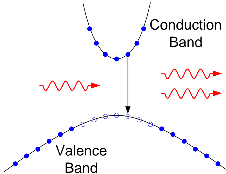
Figure 12. A simple picture of population inversion in a semiconductor.
