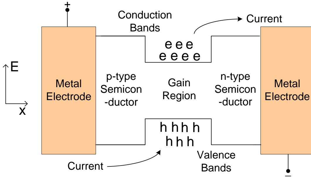
Figure 14. A double heterostructure, p-n junction for creating a population inversion in a semiconductor.
