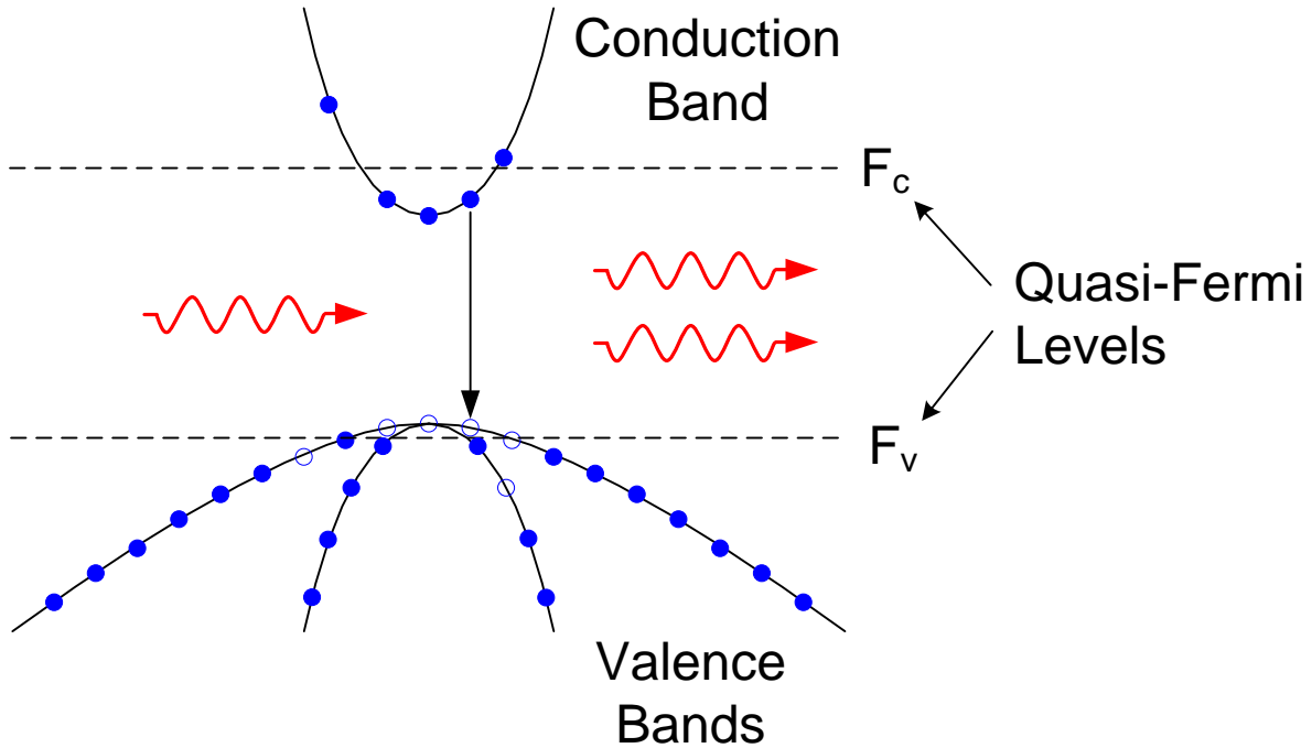
Figure 13. A more precise picture of population inversion in semiconductors includes quasi-Fermi levels.
