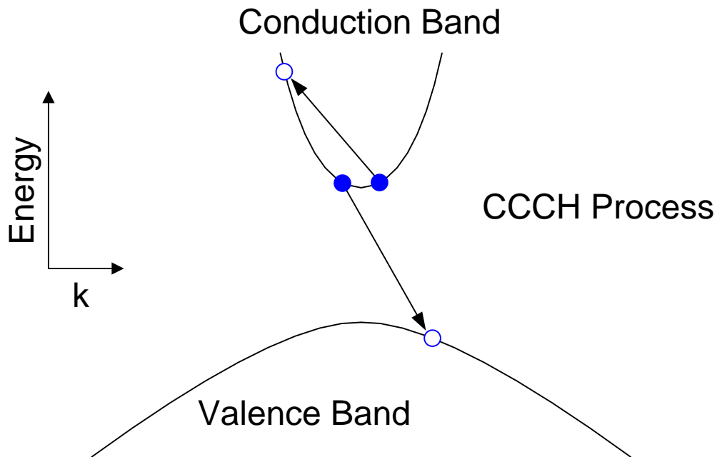
Figure 16. A CCCH Auger recombination process.
