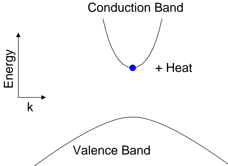
Figure 17. A CCCH Auger process removes an electron-hole pair from the semiconductor and converts the energy of the pair into heat.
