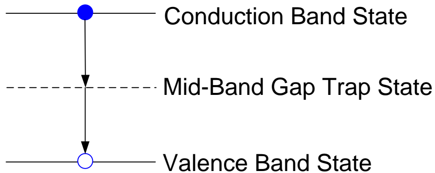
Figure 15. Shockley-Read-Hall type recombination of an electron with a hole.
