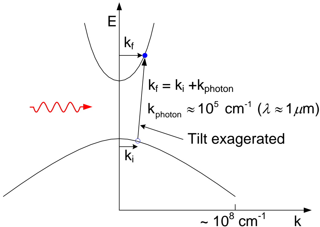
Figure 11. Optical transitions in semiconductors are “vertical”.
