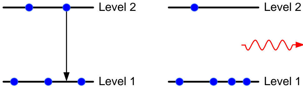
Figure 6. A particle spontaneously emits a photon.
