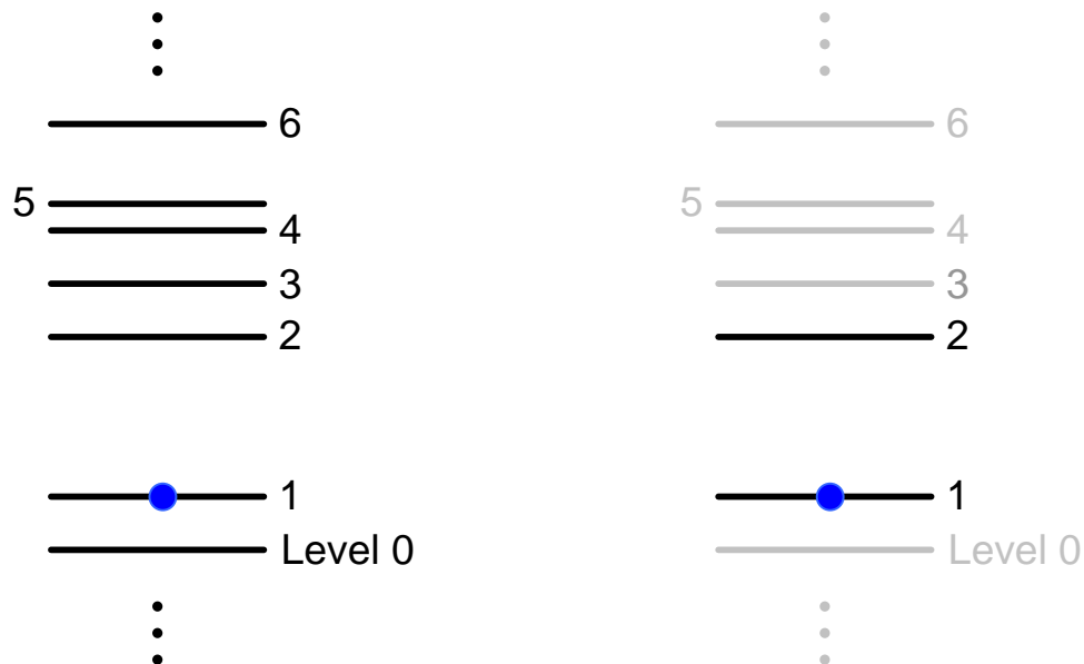
Figure 1. Energy levels for an atom or molecule. Frequently we will discuss the interaction of light with just two of the levels.
