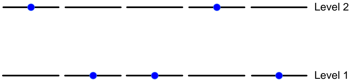
Figure 2. A collection of five particles with energies distributed between the energy levels.
