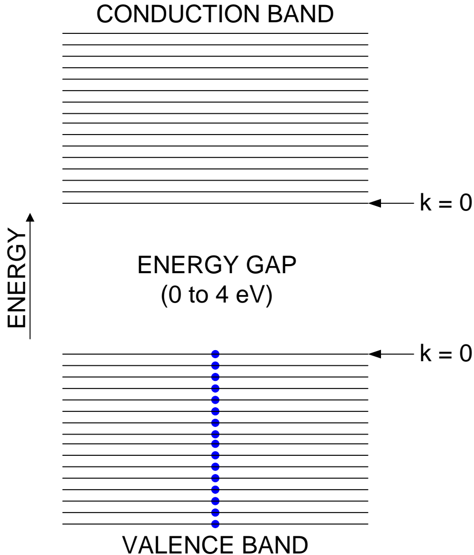
Figure 8. Energy bands in a semiconductor
