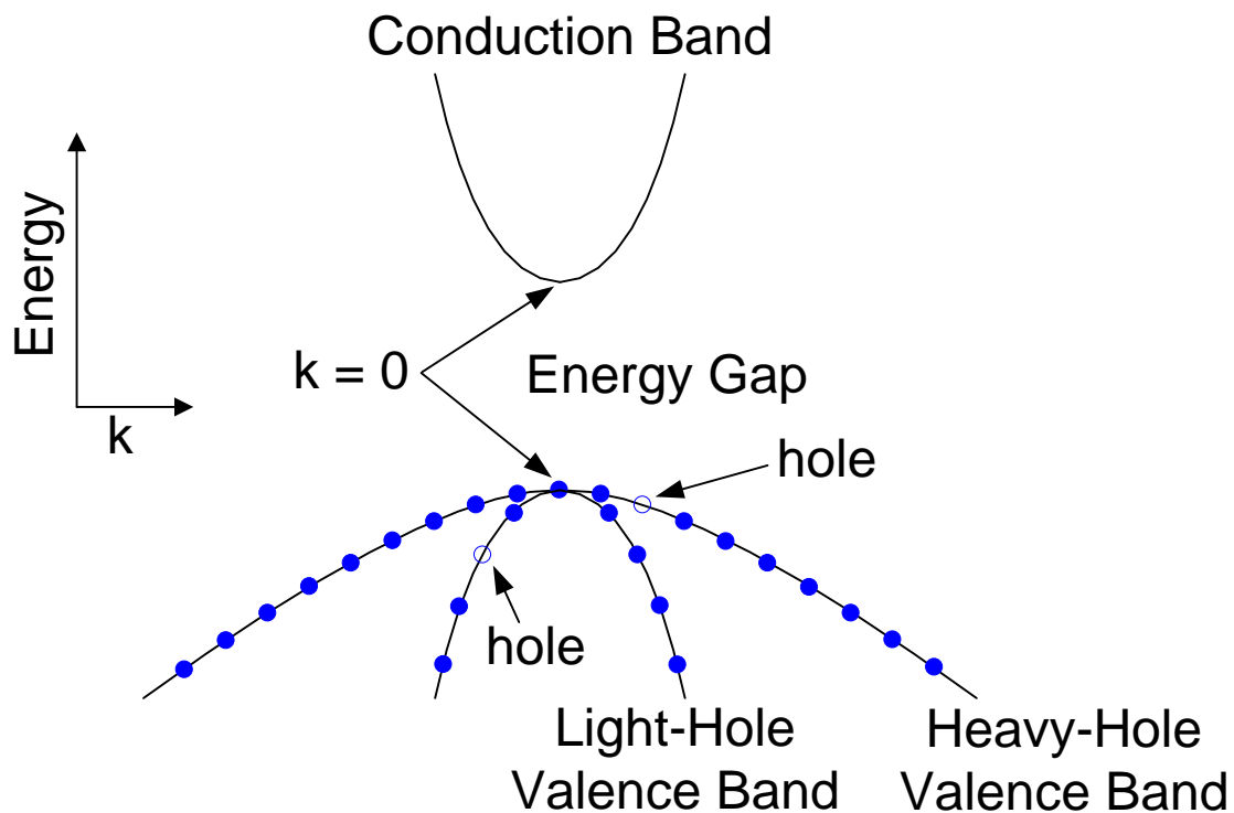
Figure 10. Energy versus momentum picture with two valence bands.
