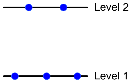
Figure 3. A shorthand version of the diagram in Figure 2.
