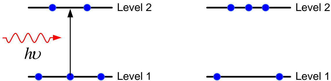
Figure 4. A photon is absorbed as a particle is excited from energy level 1 to energy level 2.
