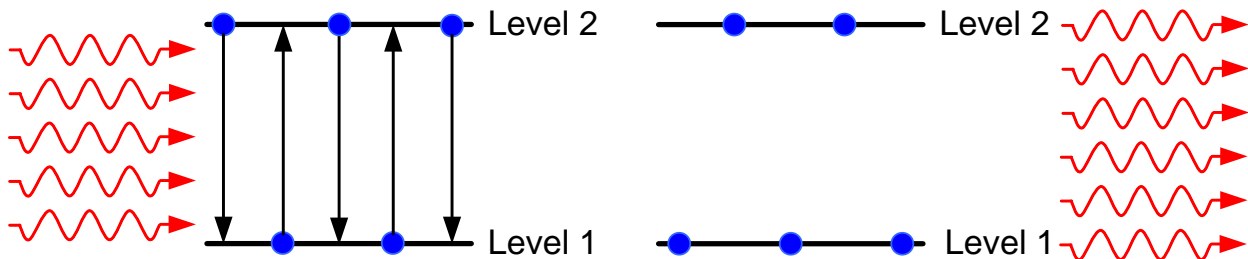
Figure 7. An “inverted” population amplifies light.
