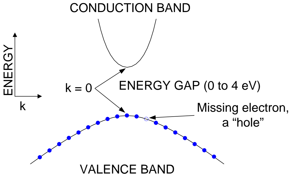
Figure 9. Valence and conduction bands in the energy versus momentum picture.
